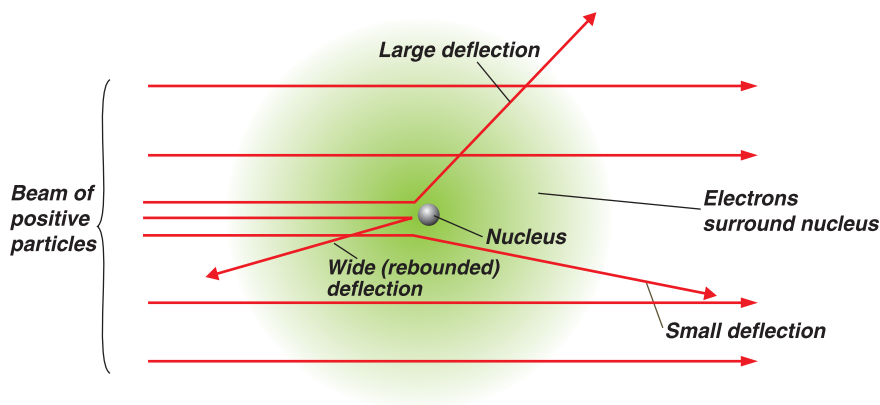
Figure 1.4 Rutherford's \alpha – particles experiment.
